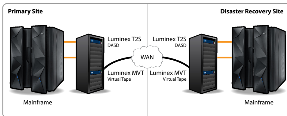
Typical production and remote disaster recovery configuration with Luminex T2S and MVT.
